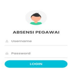
Gambar 1. Form Login
